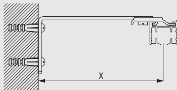
0829 Wall Bracket (2 3/4")
